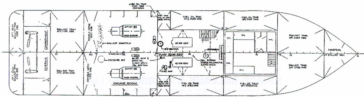
HOLD PLAN
