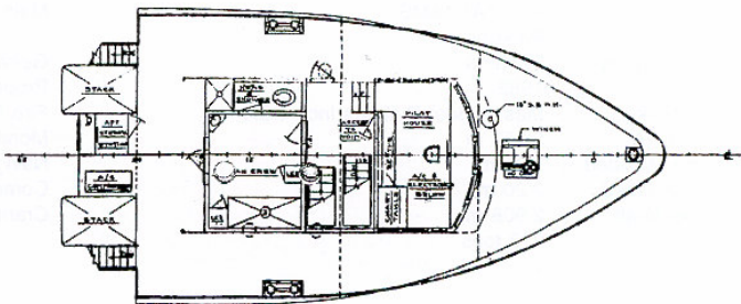
FOCSLE DECK
