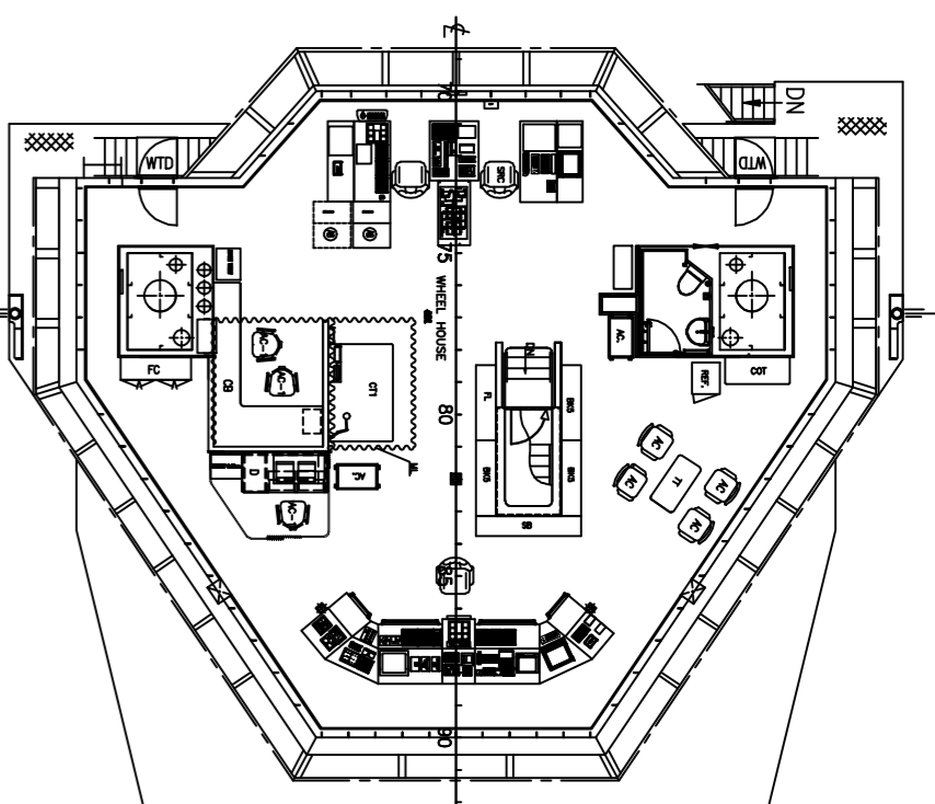
NAV. BRIDGE DECK
