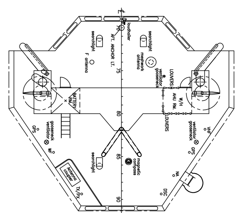
COMPASS DECK
